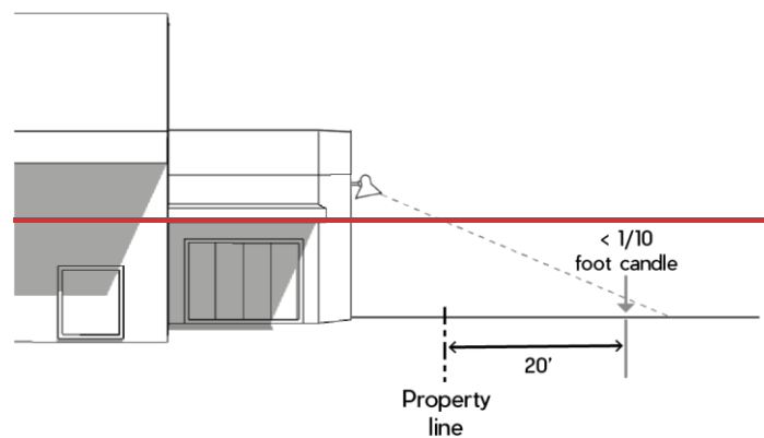
Figure 4-6: Light Trespass
