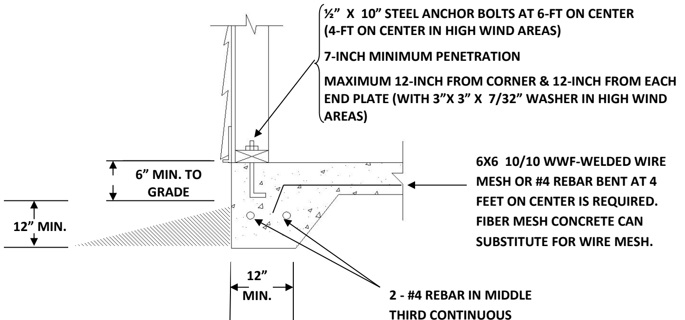
Figure: Unheated Monolithic Foundation Details
