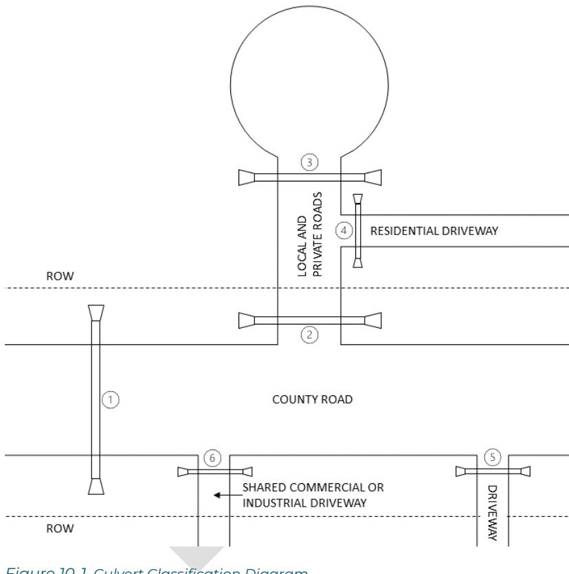
Figure 10-1. Culvert Classification Diagram
