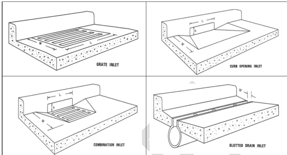
Figure 8-1: Perspective view of different inlet types
